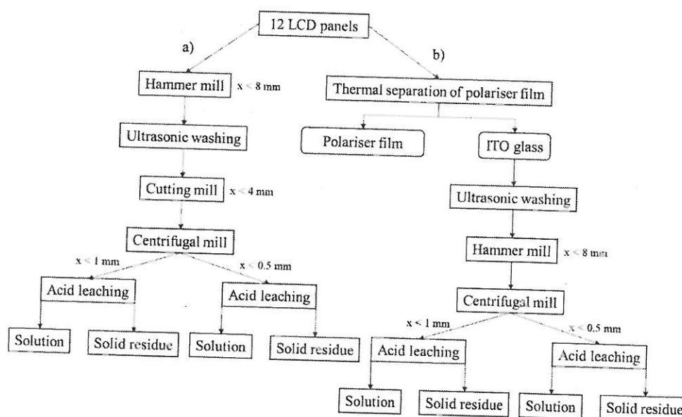
Figure 2 The processing flowsheet of LCD panels a) with and b) without polarising film
