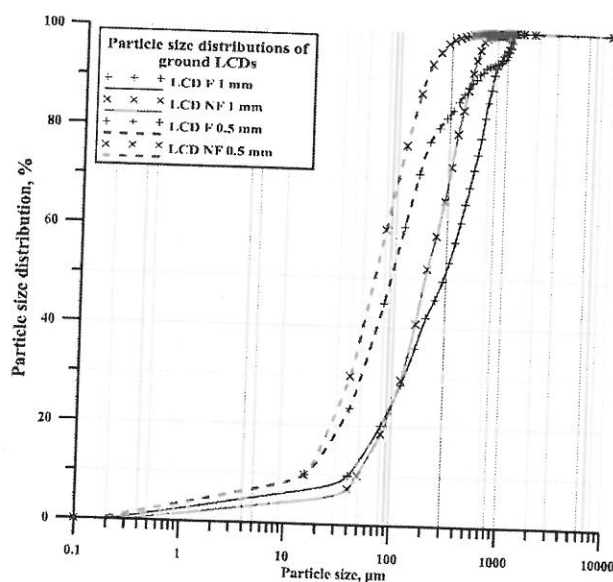
Figure 7 The particle size distributions of the LCDs ground in centrifugal mill
