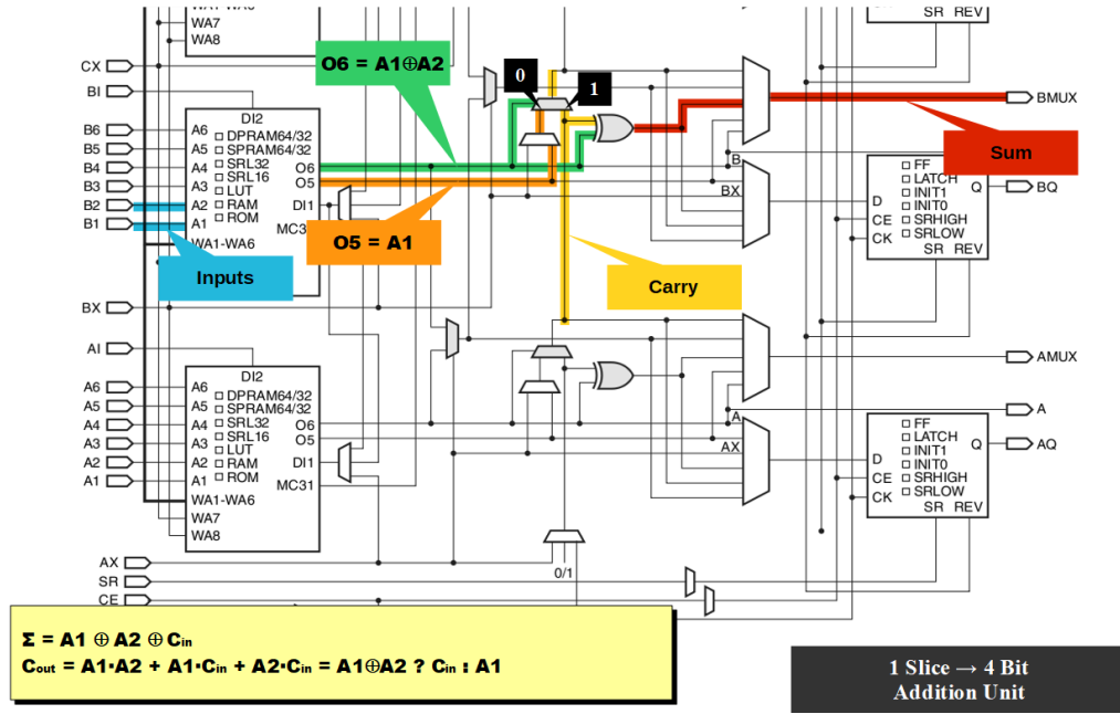
Figure 17.11: Realizing an adder.
