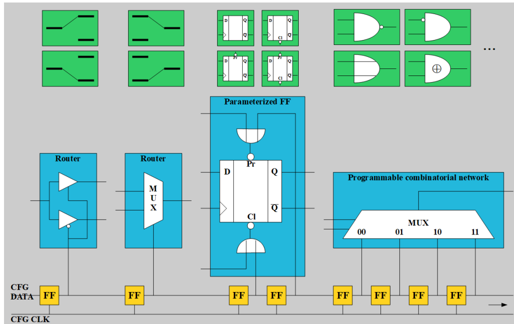
Figure 17.7: How programmable hardware is constructed.
