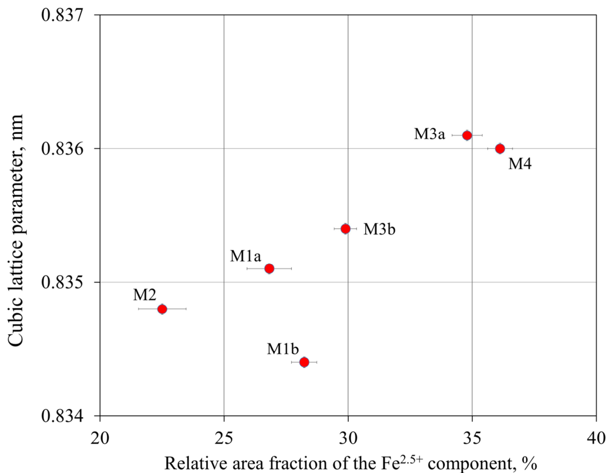
Figure 10. The cubic lattice parameter of the prepared samples depicted as a function of the relative area fraction of the \text{Fe}^{2.5+} component as determined on the basis of room-temperature Mössbauer spectra (Figure 7). See Table 1 and Figure 3 for corresponding data. Error bars refer to the standard error of the data.
