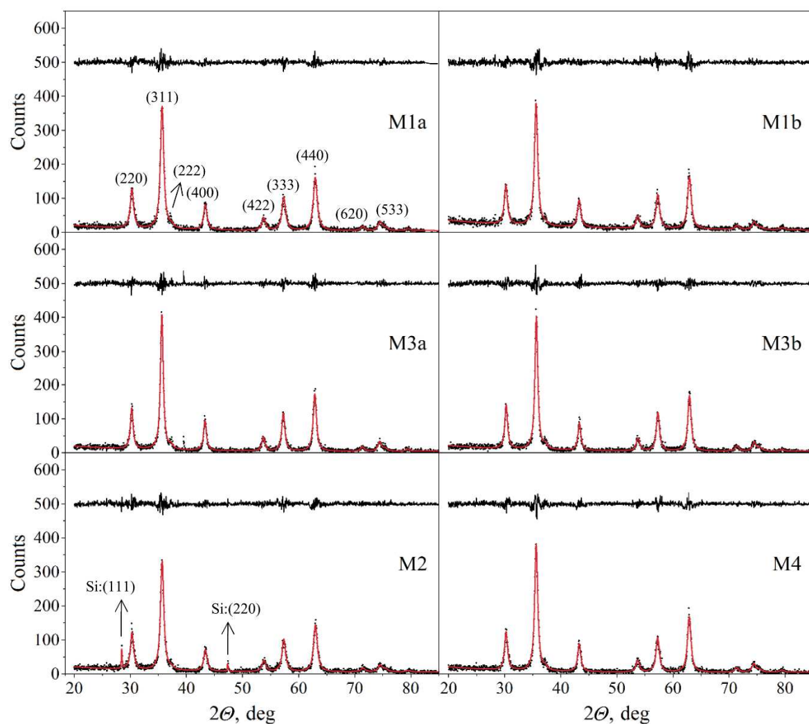
Figure 2. Powder X-ray diffractograms of the prepared samples (recorded with Cu K_{\alpha} radiation) along with the corresponding fitting curves, with the cubic spinel (hkl) indexes indicated in the case of M1a. Silicon powder was mixed with sample M2 in order to calibrate the 2\theta axis. Above the diffractograms the respective fit residuals are displayed. The sharp peak at 2\theta = 39.5 deg, observed only for M3a, remained unidentified and is regarded as an artifact.
