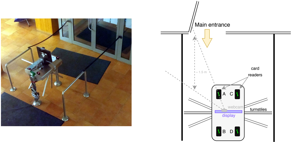
Figure 2.1: Photo and detailed plan view of the access control system at the main entrance.
