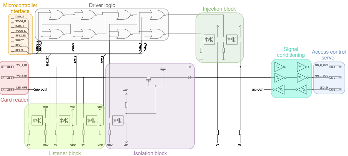
Figure 2.4: Overview of the main parts of the custom board. Driver logic instructs insulation block to separate card reader from the access control server and allows injection block to send data to Wiegand bus, but only when appropriate enabling signals are coming from the microcontroller. Listener block forwards signals coming from card reader to microcontroller. Signal conditioning components compensates effect of listener, insulation and injection blocks.
