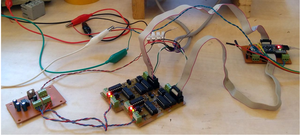
Figure 2.3: Symmetric power supply (left), two custom boards (middle) and microcontroller (right). The symmetric power supply gets energy from the same source as the card readers and feeds 0V, +5V and -5V to the custom boards. Custom boards listens and injects card IDs to Wiegand buses (blue and white wires entering custom boards from the right). Microcontroller are connected to both custom boards. It relays data between the custom board and Edge and also encodes and decodes card IDs going to and coming from Wiegand interface.
