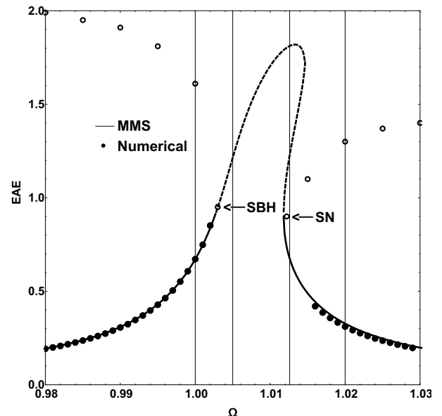
Fig. 7. Bifurcation diagram (or resonance curve), where SBH corresponds to subcritical Hopf bifurcation and SN to saddle-node bifurcation.
