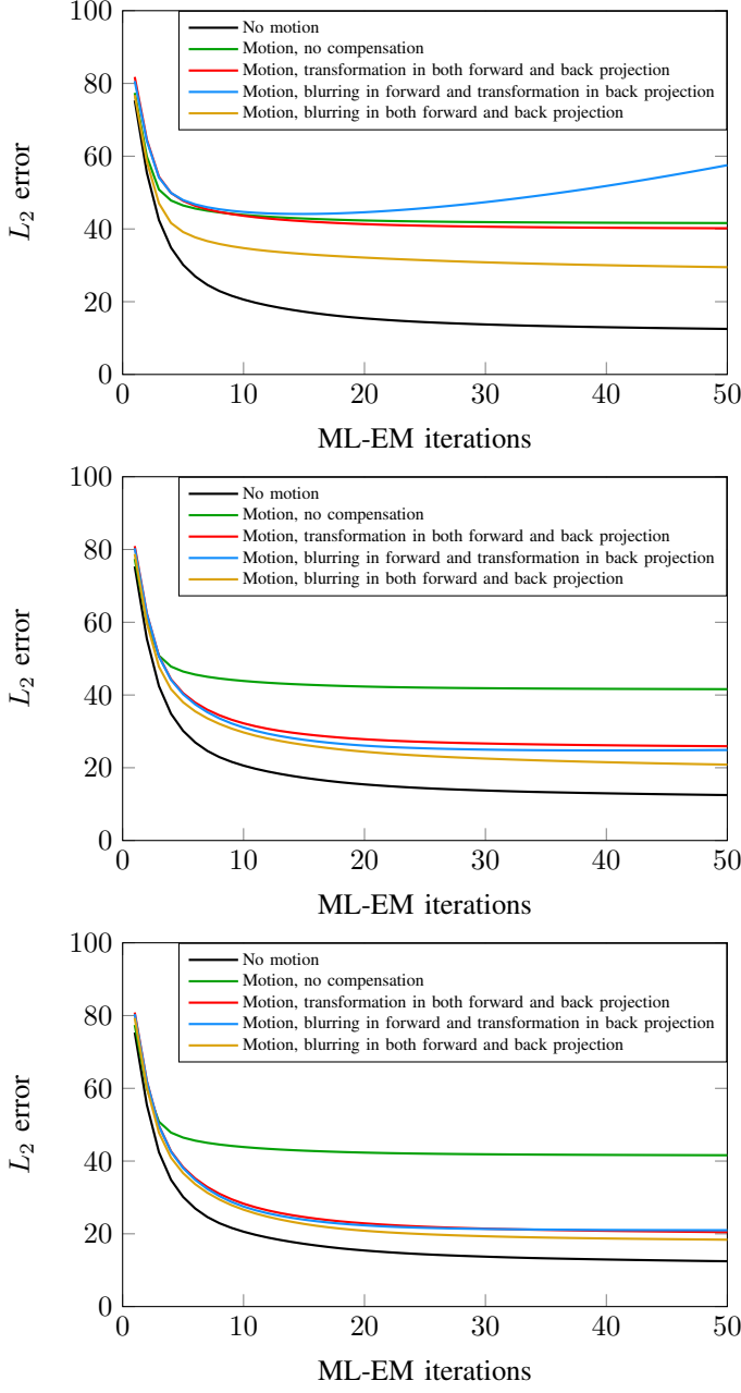
Fig. 4: L_2 error curves of the 2D brain phantom as a function of the number of ML-EM iterations, when the measurement time is decomposed into 1, 2, and 3 frames
