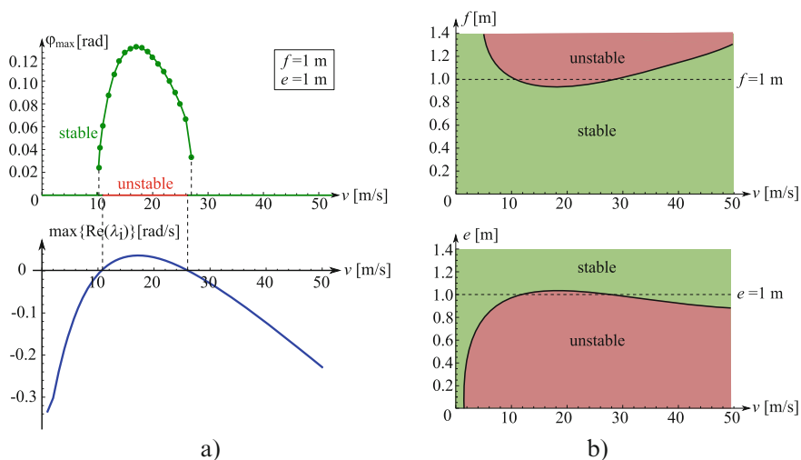
Fig. 7 (a) The bifurcation diagram of the four degree-of-freedom system, in case of k = 75,000 N/m (top panel) and the real part of the rightmost characteristic root of the linearized system (bottom panel). (b) The effects of parameters f and e on the linear stability of the rectilinear motion. The green areas correspond to linearly stable, the red areas correspond to linearly unstable motion
