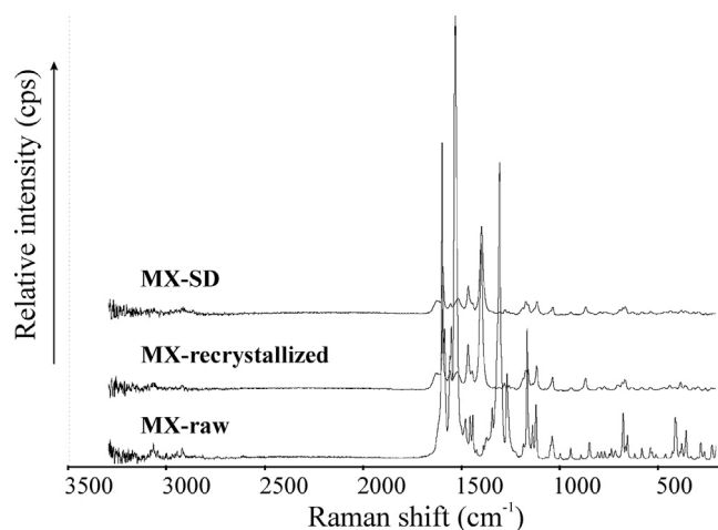
Fig. 1. Raman spectra of the raw MX (MX-raw), MX dissolved in sodium hydroxide at 1.5 mg/mL and dried out at 40 °C, 24 h (MX-recrystallized) and spray dried MX (MX-SD).
