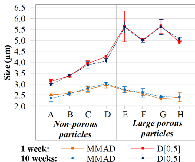
Fig. 5. Comparison of the aerodynamic and geometric diameter (MMAD = mass median aerodynamic diameter and D[0.5] = median geometric diameter) of the spray dried formulations. Data show the low density LPPs (E: MX/LEU/HA 0.3 /AB 1.5 , F: MX/LEU/HA 0.15 /AB 1.5 , G: MX/LEU/HA 0.3 /AB 2 and H: MX/LEU/HA 0.15 /AB 2 ) have the same or smaller MMAD than smaller but denser non-porous particles (A: MX-SD, B: MX/LEU, C: MX/LEU/HA 0.3 and D: MX/LEU/HA 0.15 ). Data are represented as mean \pm S.D., n = 3.
