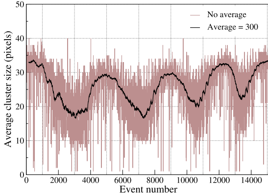
Fig. 3. Average cluster size versus event number. Here the event number is the trigger id for each time frame of about 10 \mu s. The scan time increases with the increase in the event number while the beam position changed.
