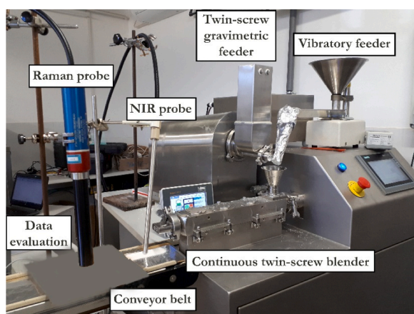
Fig. 7. Photo of the continuous blending experimental setup.
