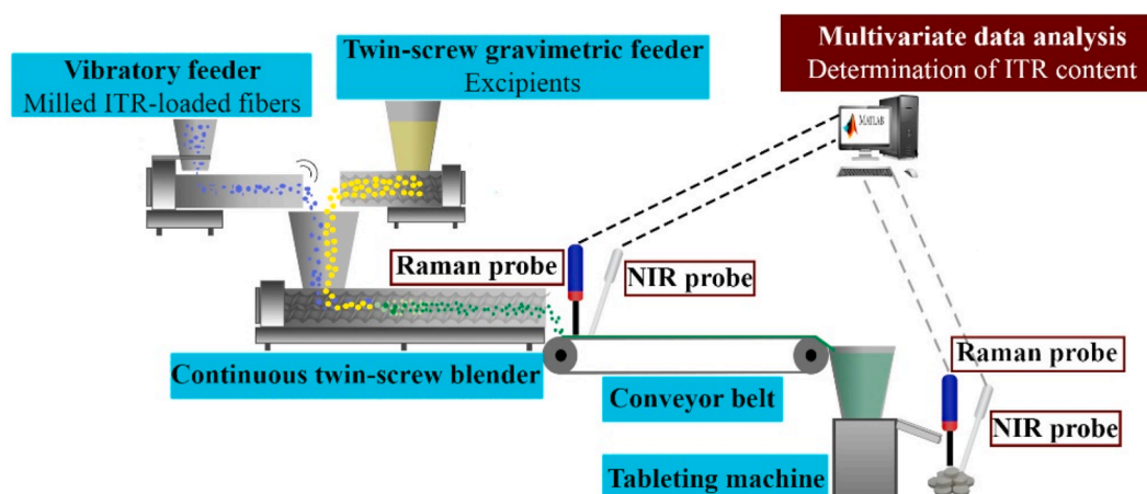
Fig. 2. Schematic illustration of the continuous experimental set-up.
