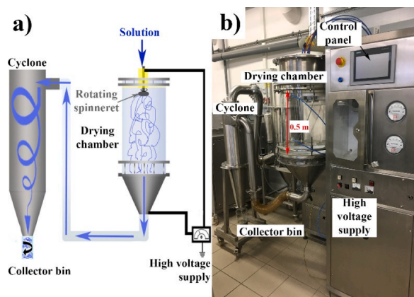
Fig. 1. Schematic drawing (a) and photo (b) of the applied high speed electrospinning (HSES) apparatus connected with a cyclone.
