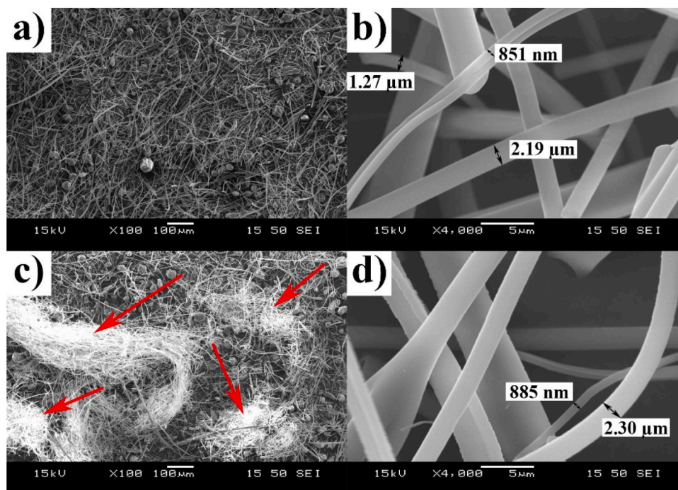
Fig. 3. Scanning electron microscopic images of the prepared electrospun sample a) before milling ( 100 \times magnification); b) before milling ( 4000 \times magnification); c) after milling ( 100 \times magnification) (red arrows indicate the entangled fibers); d) after milling ( 4000 \times magnification).
