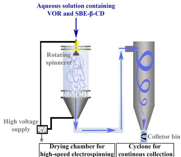
Fig. 1. Schematic design of the applied high-speed electrospinning apparatus coupled with a cyclone.
