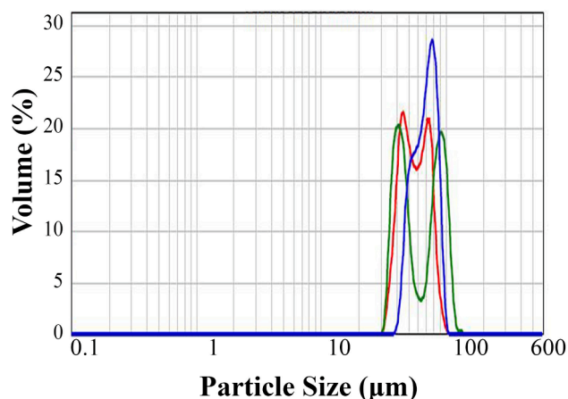
Fig. 3. Particle size distribution of O1.5 samples. (Different colors indicate three repeated measurements. The x-axis is depicted in logarithmic scale.)
