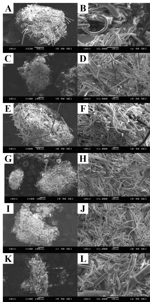
Fig. 2. Morphology of the fibers after milling (A-B: O0.8 sample; C-D: O1.5 sample; E-F: O2.0 sample; G-H: C1.5 sample; I-J: C2.0 sample; K-L: H1.0).
