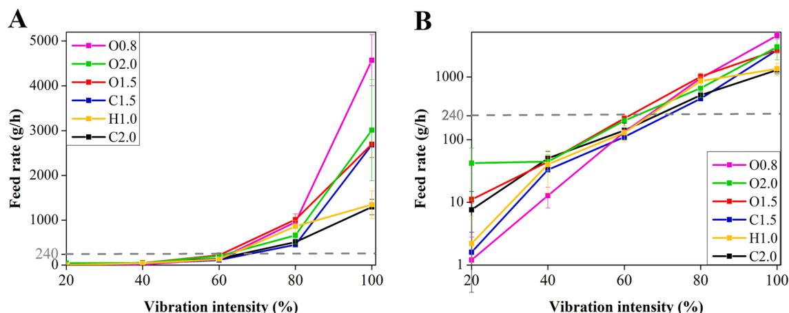
Fig. 6. Correlation between the feed rate and the intensity of vibratory amplitude represented on the original scale (a) and logarithmic scale (b).
