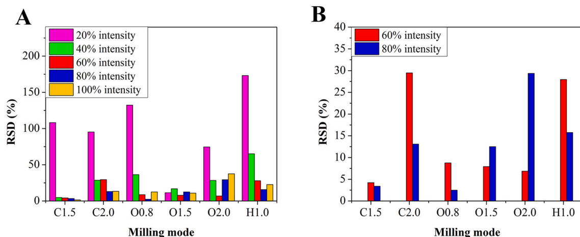
Fig. 7. RSD values at different vibratory intensities.
