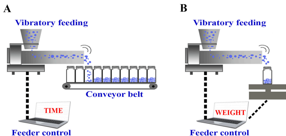
Fig. 9. Vial filling based on time-control (a) and weight-control (b).
