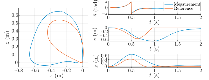
Fig. 8. Backflipping measurement results with geometric control. The trajectories show that the maneuver is performed successfully, and the drone gets back to the initial position at the end.
