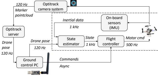
Fig. 5. Block diagram of the experimental setup: indoor quadcopter navigation with internal and external measurement system.
