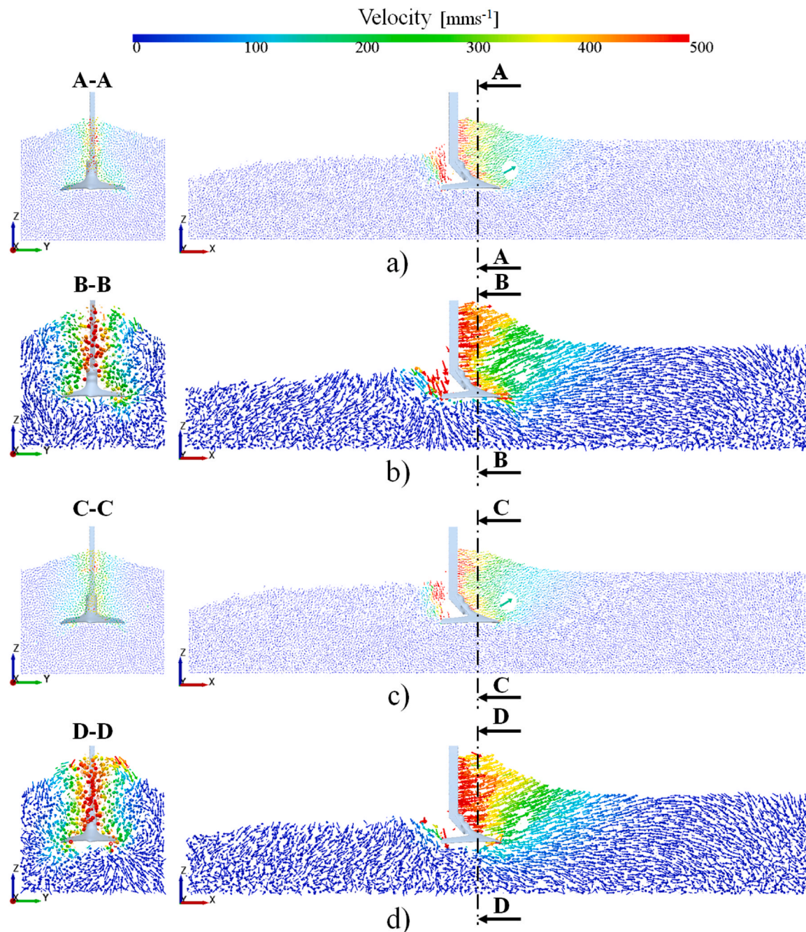
Fig. 17. Velocity field of particles in the soil sweep tool simulations at 1.5 m tool displacement in the case of a) spherical particles with 2900 \text{ kgm}^{-3} density, b) clump particles with 2900 \text{ kgm}^{-3} density, c) spherical particles with 2000 \text{ kgm}^{-3} density, and d) clump particles with 2000 \text{ kgm}^{-3} density.
