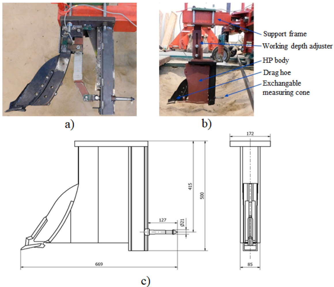
Fig. 1. Horizontal penetrometer a) internal structure, b) parts and c) inclusion dimensions of measuring device (dimensions are in mm).
