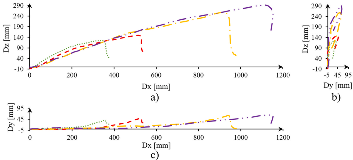
Fig. 15. Trajectory path of the displacement sensor in the case of HP — measurement and simulations of -- spherical particles with 2900 \text{ kgm}^{-3} density, -- clump particles with 2900 \text{ kgm}^{-3} density, ... spherical particles with 2000 \text{ kgm}^{-3} density and -- clump particles with 2000 \text{ kgm}^{-3} density, projection of the trajectories to the a) x-z plane, b) y-z plane and c) x-y plane.
