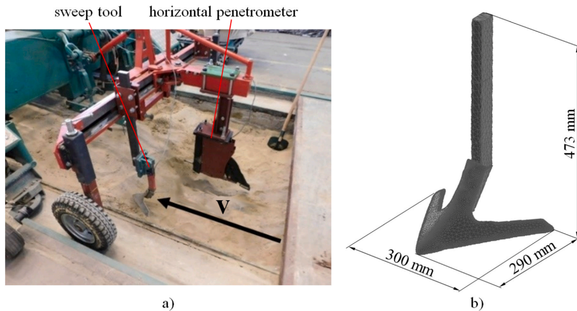
Fig. 3. Soil sweep tool measurement, a) initial state of the sweep tool and the HP (the direction of the measurement is indicated by the velocity vector v ), b) inclusion dimensions of the sweep tool.
