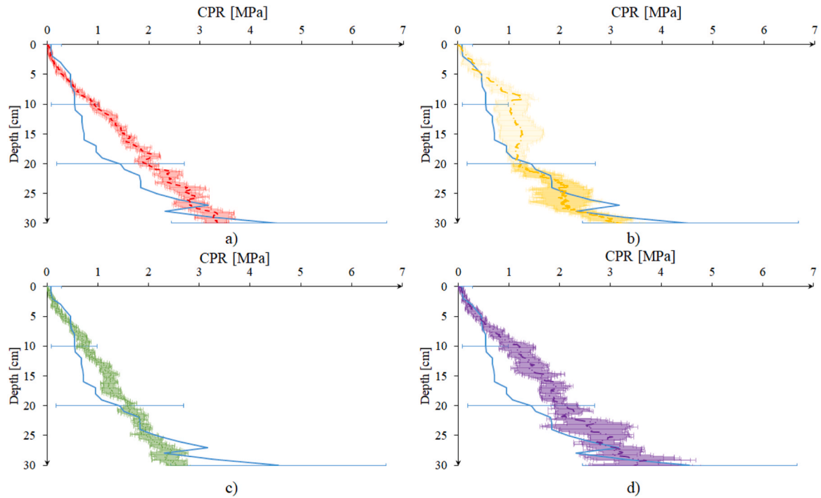
Fig. 19. Vertical CPR in the function of soil depth in the case of – measurements and simulations of a) – spherical particles with 2900 kgm -3 density, b) - - clump particles with 2900 kgm -3 density, c) ··· spherical particles with 2000 kgm -3 density and d) - · - clump particles with 2000 kgm -3 density.
