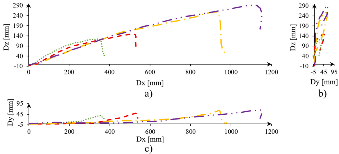
Fig. 18. Trajectory paths of the displacement sensor in the case of soil sweep interaction simulations of -- spherical particles with 2900 kgm -3 density, - - clump particles with 2900 kgm -3 density, ··· spherical particles with 2000 kgm -3 density and - · - clump particles with 2000 kgm -3 density, projection of the trajectories to the a) x-z plane, b) y-z plane and c) x-y plane.
