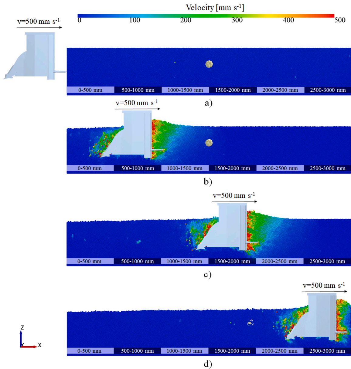
Fig. 9. Velocity of the assembly with spherical particle shape and 2900 \text{ kgm}^{-3} density at a) 0 mm, b) 1000 mm, c) 2000 mm and d) 3000 mm HP displacement (the velocity of the HP is indicated by vector \mathbf{v} ).
