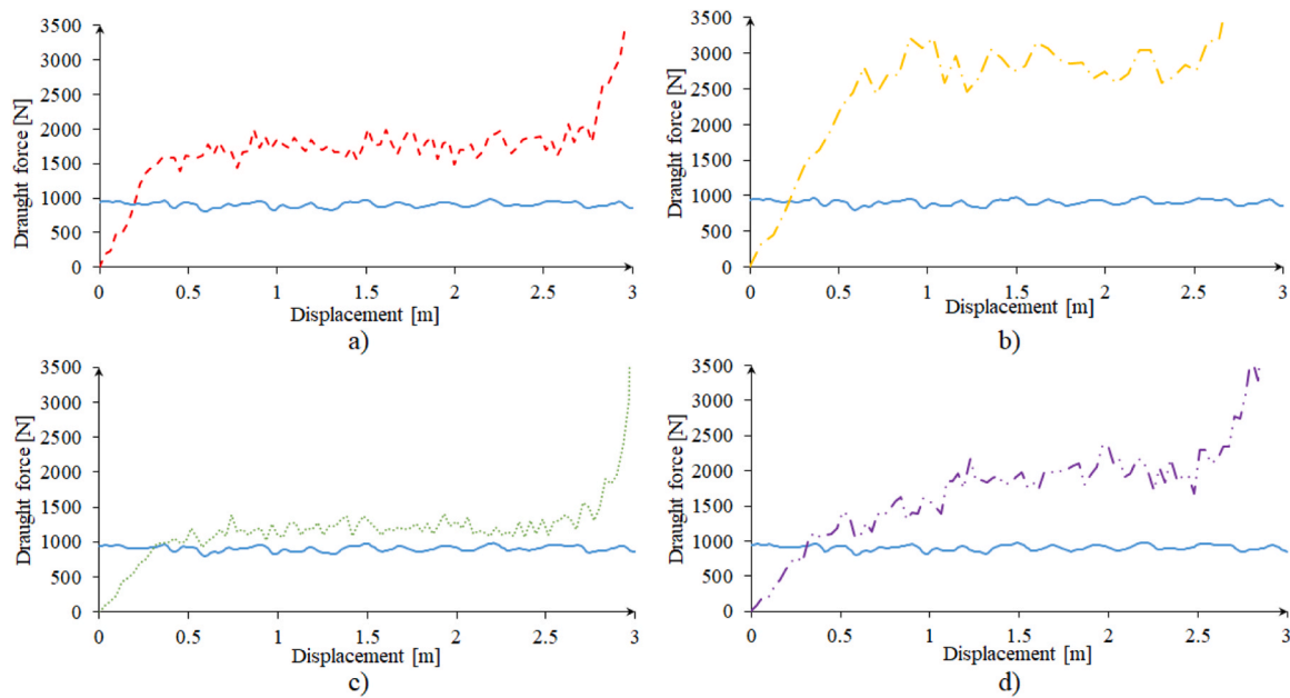
Fig. 16. Draught force acting on the sweep tool in the function of tool displacement in the case of — measurement and simulations of a) -- spherical particles with 2900 \text{ kgm}^{-3} density, b) -- clump particles with 2900 \text{ kgm}^{-3} density, c) ... spherical particles with 2000 \text{ kgm}^{-3} density and d) -- clump particles with 2000 \text{ kgm}^{-3} density.
