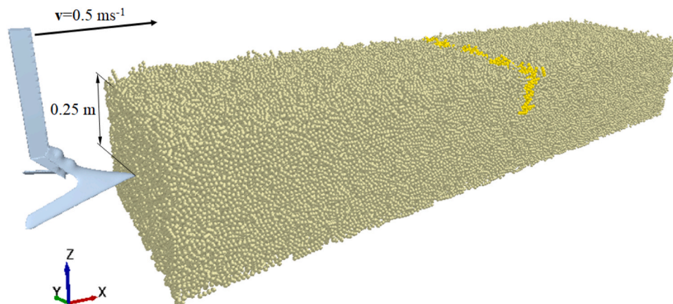
Fig. 7. Initial state of the soil sweep interaction in the case of the clump particle assembly (the velocity of the tool is indicated by vector \mathbf{v} ).
