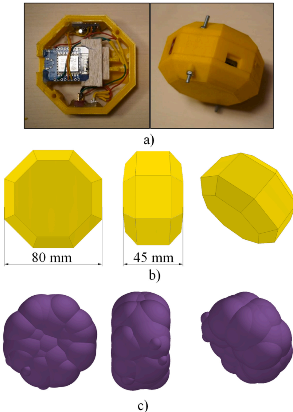
Fig. 5. Displacement sensor a) photo, b) CAD model, c) clump model built up from spheres.
