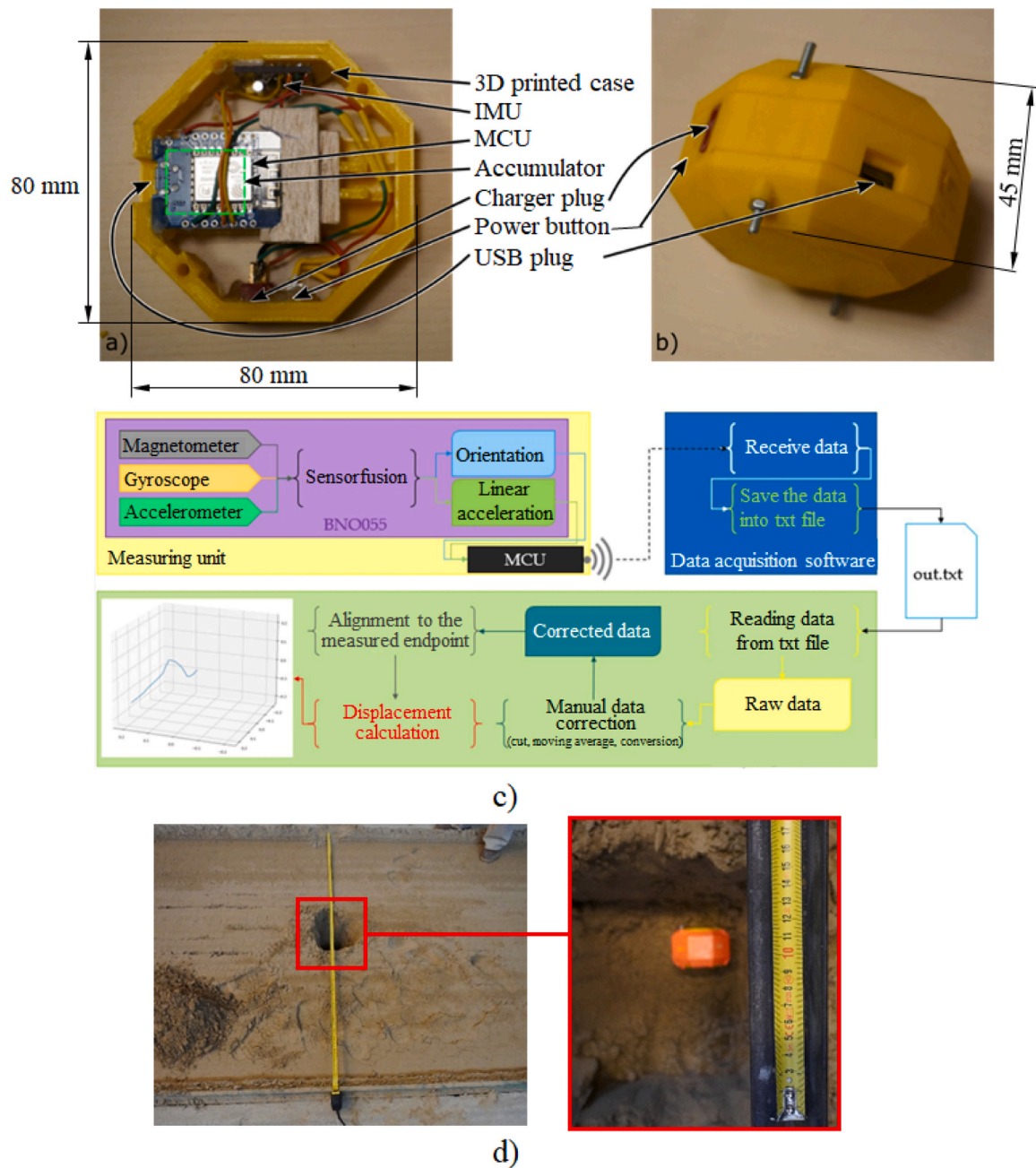
Fig. 2. Displacement sensor, a) internal and b) external structure, c) flowchart of data extraction and processing, d) placement in the soil.
