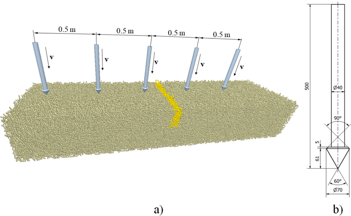
Fig. 8. Simulation of the vertical penetrometer measurement, a) initial state in the case of the clump assembly (the velocity of the penetrometer is indicated by vector v ), b) geometry and sizes of the penetrometer used in the simulations (dimensions are in mm).
