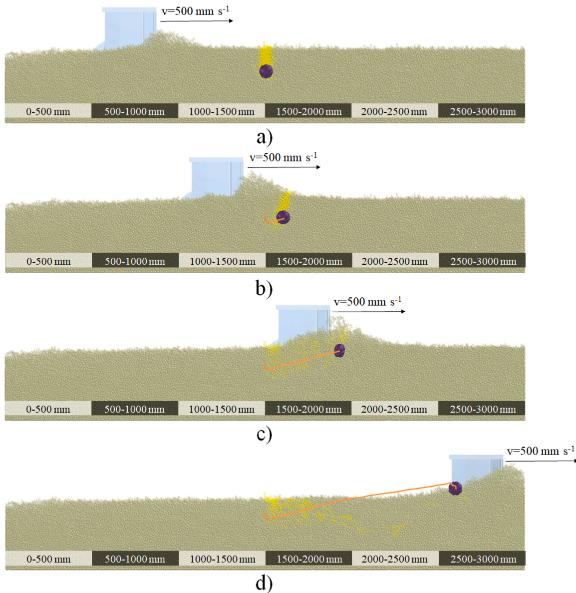
Fig. 13. Movement of the displacement sensor in the simulation of the HP measurement with clump particle shape and 2900 \text{ kg m}^{-3} density at a) 1000 mm, b) 1500 mm, c) 2000 mm, d) 3000 mm HP displacements (due to the visibility of the displacement sensor, the soil particles and the HP were made 90 % transparent, the velocity of the HP is indicated by vector v , the trajectory path of the displacement sensor is indicated by an orange line, and the particles which were initially above the displacement sensor are coloured yellow).
