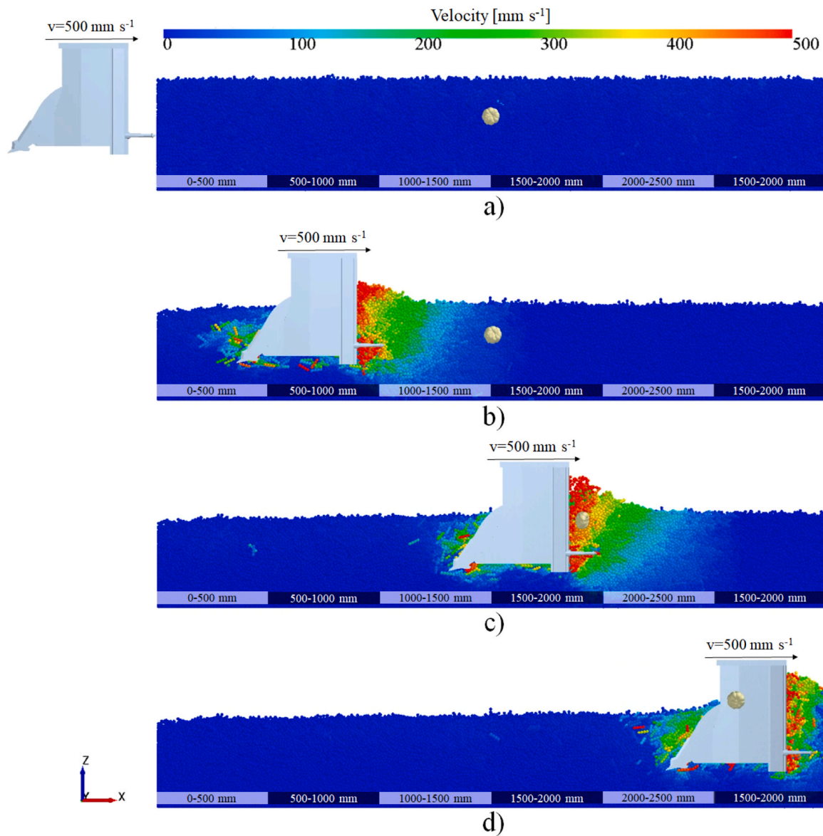
Fig. 12. Velocity of the assembly with clump particles with 2900 \text{ kg m}^{-3} density at a) 0 mm, b) 1000 mm, c) 2000 mm and d) 3000 mm HP displacement (the velocity of the HP is indicated by vector \mathbf{v} ).
