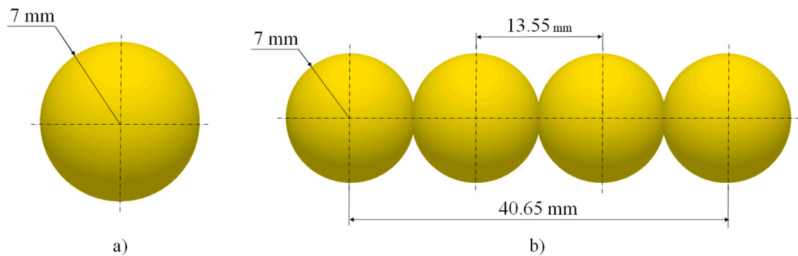
Fig. 4. Particles used for soil modelling, a) spherical particle, b) clump particle built up from 4 spheres.
