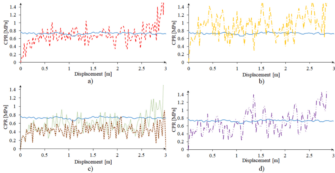
Fig. 14. Horizontal CPR in the function of HP displacement in the case of — measurements and simulations of a) -- spherical particles with 2900 \text{ kgm}^{-3} density, b) -- clump particles with 2900 \text{ kgm}^{-3} density, c) ... spherical particles with 2000 \text{ kgm}^{-3} density, -- spherical particles with 2000 \text{ kgm}^{-3} density with the HP body removed and only the cone present and d) -- clump particles with 2000 \text{ kgm}^{-3} density.
