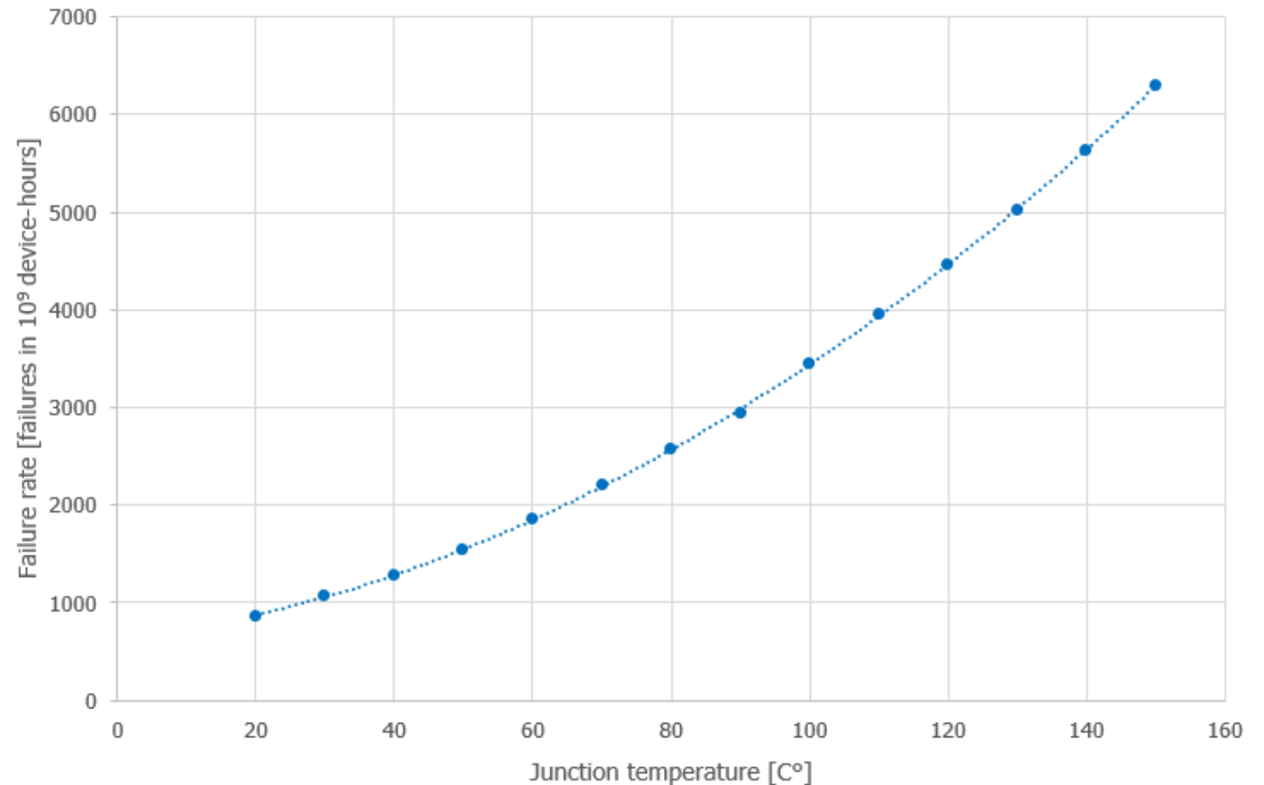
Failure Rate of MOSFET
