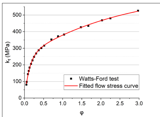
Figure 4. Watts-Ford test result and flow curve fitted to the data.
