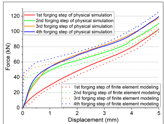
Figure 7. Comparison of force-displacement curves resulting from physical simulation and finite element modeling.
