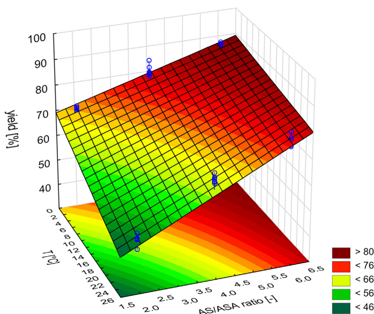
Fig. 4. Response Surface presenting yield as a function of temperature and antisolvent to ASA solution ratio in the investigated experimental region.
