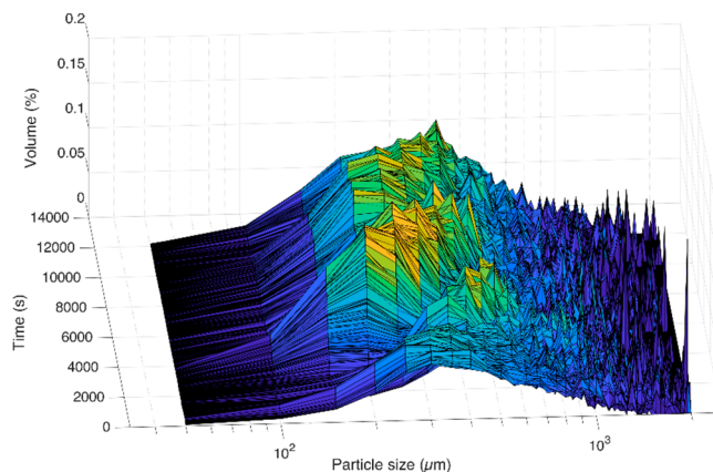
Figure 12. Result of continuous in-line image analysis of continuous MSMPR crystallization. A new CSD was calculated every 30 s from the detected crystals in the captured images.
