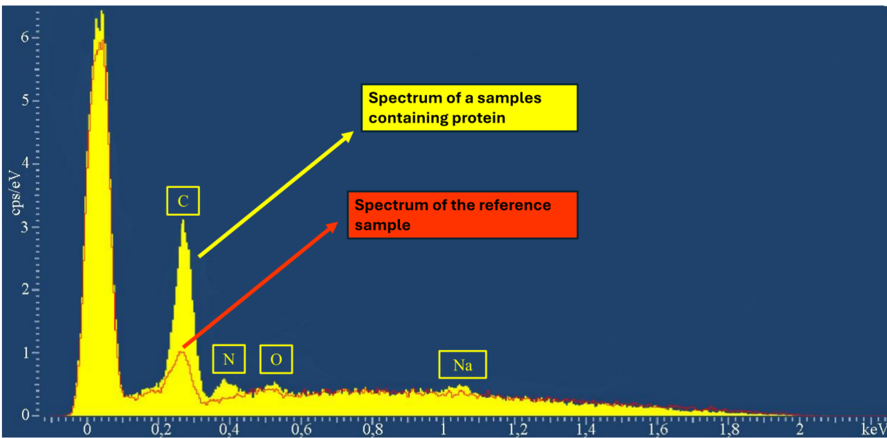
Comparison of protein covered and untreated surfaces by energy dispersive X-ray spectroscopy.
