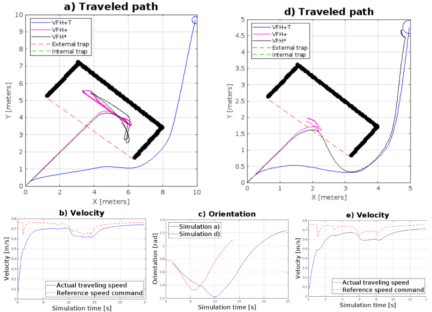
Fig. 7. Quantitative analysis of pathfinding algorithms in U-shaped obstacles of VFH + T, VFH+, and VFH* algorithms. a): Trajectory optimization in U-shaped obstacles: comparative path analysis of VFH + T, VFH+, and VFH* with emphasis on loop avoidance and path efficiency. b): Velocity profile metrics of the VFH + T trajectory depicted on Fig. 7/a. c): Orientation metrics across simulated trials, angular displacement analysis reflecting algorithmic response to navigational challenges. d): Enhanced obstacle proximity detection: VFH + T algorithm's early recognition and avoidance strategies reducing path length by 17 % relative to VFH*. e): Graphical depiction of actual vs. commanded speed during simulation of VFH + T trajectory illustrated on Fig. 7/d.
