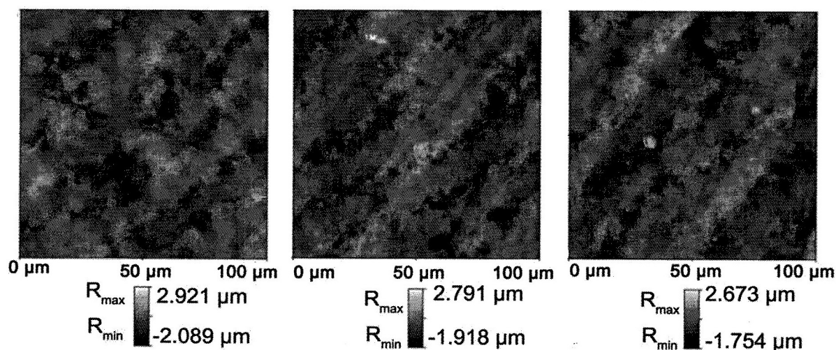
Fig. 8. Topographic pictures of heat treated samples under standard atmosphere with 1-2-3 reflows
