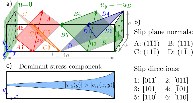
Fig. 1. a) Considered system geometry and the slip planes of the FCC sample. b) Specific vectors corresponding to the slip planes and the BVs. c) The schematics highlights with blue the region on the front face of the cantilever where the shear stresses are larger than the compressive stresses.
