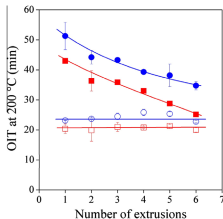
Fig. 9. Effect of the number of extrusions on the residual thermo-oxidative stability of polyethylene stabilised with 1000 ppm curcumin (○), 1000 ppm curcumin + 2000 ppm P-EPQ (●), 1000 ppm I1010 (□), and 1000 ppm I1010 + 2000 ppm P-EPQ (■).
