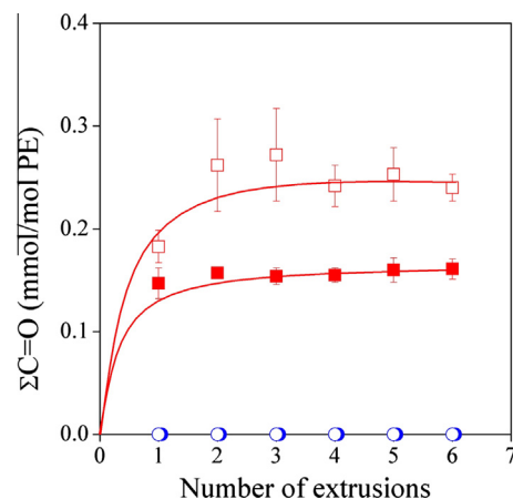
Fig. 6. Effect of the number of extrusions on the carbonyl group content of polyethylene stabilised with 1000 ppm curcumin (○), 1000 ppm curcumin + 2000 ppm P-EPQ (●), 1000 ppm I1010 (□), and 1000 ppm I1010 + 2000 ppm P-EPQ (■).
