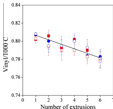
Fig. 5. Effect of the number of extrusions on the vinyl group content of polyethylene stabilised with 1000 ppm curcumin (○), 1000 ppm curcumin + 2000 ppm P-EPQ (●), 1000 ppm I1010 (□), and 1000 ppm I1010 + 2000 ppm P-EPQ (■).
