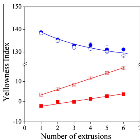
Fig. 10. Effect of the number of extrusions on the yellowness index of polyethylene stabilised with 1000 ppm curcumin (○), 1000 ppm curcumin + 2000 ppm P-EPQ (●), 1000 ppm I1010 (□), and 1000 ppm I1010 + 2000 ppm P-EPQ (■).
