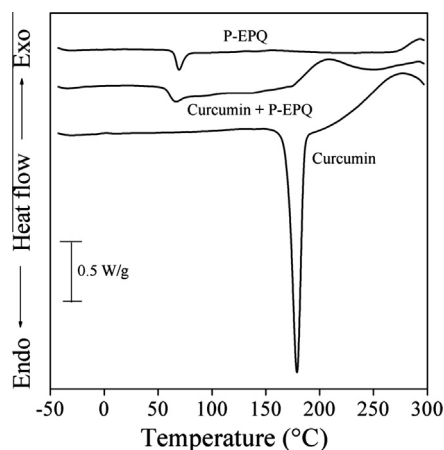
Fig. 1. Thermograms (melting) of curcumin, P-EPQ, and a 1:1 mixture of curcumin and P-EPQ measured under nitrogen after melting in Ar atmosphere at 220 °C for 1 min and then cooling down to ambient temperature. Heating rate: 10 °C/min.
