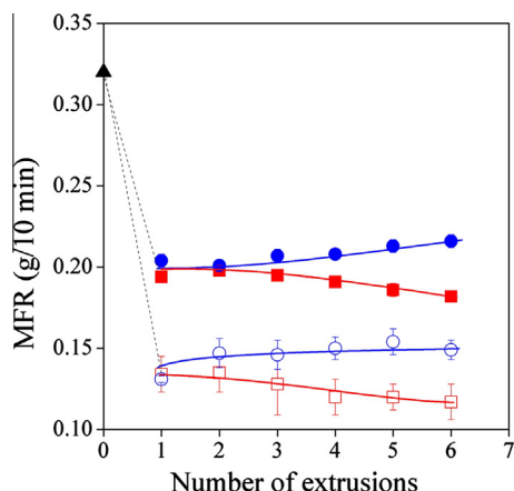
Fig. 7. Effect of the number of extrusions on the melt flow rate of polyethylene stabilised with 1000 ppm curcumin (○), 1000 ppm curcumin + 2000 ppm P-EPQ (●), 1000 ppm I1010 (□), and 1000 ppm I1010 + 2000 ppm P-EPQ (■) Neat powder (▲).
