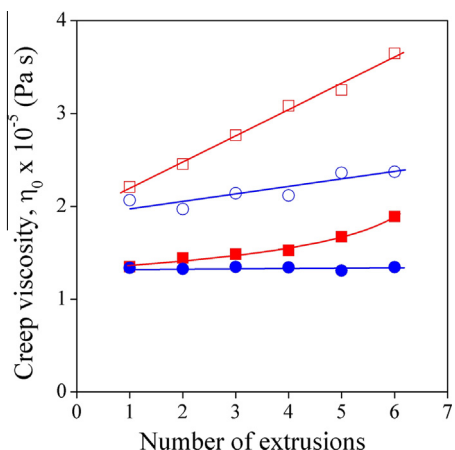
Fig. 8. Effect of the number of extrusions on the creep viscosity of polyethylene stabilised with 1000 ppm curcumin (○), 1000 ppm curcumin + 2000 ppm P-EPQ (●), 1000 ppm I1010 (□), and 1000 ppm I1010 + 2000 ppm P-EPQ (■).
