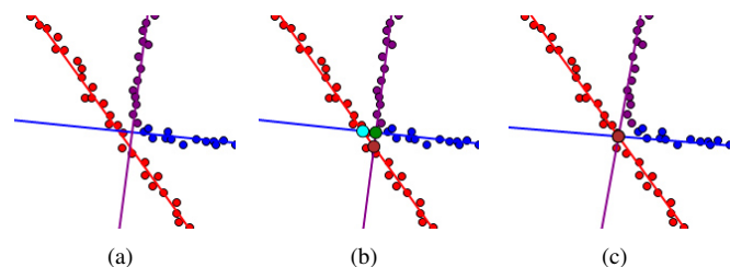
Fig. 5. Three lines meet at a common point: (a) initial state; (b) pairwise intersection (auxiliary points); and (c) “three points are equal” constraint enforced.
